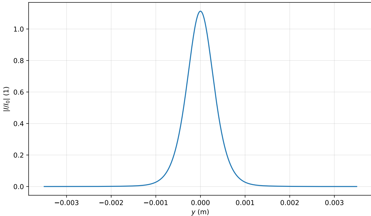
Intensity profile I(x=0, y, z=2.946)/I_0 , P_{in}=0.8P_{cr} , artificial time
